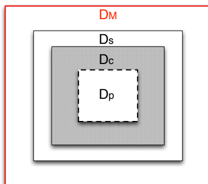
Figure 1: Domains: D_p is the zone to be protected, D_c is the domain of sensors, D_s is the domain of sources, and D_M is the modeled domain.
